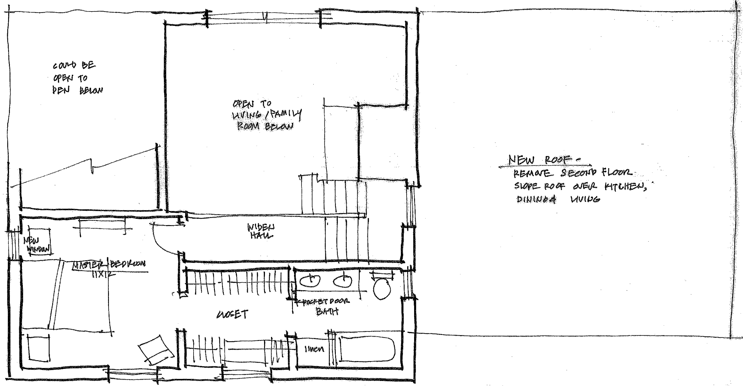
2248 LEHIGH - SUGGESTED RENOVATIONS UPPER LEVEL 1/4" = 1'0" DIMENSIONS APPROXIMATE
